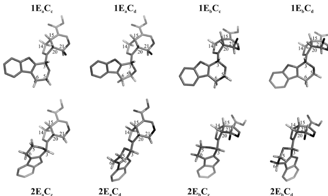
Figure 1. Structures of the conformations obtained by RM1 for psychollatine ( 1 ) and for croceaine A ( 2 ). 7 With the exception of the hydrogen atoms attached to C-3, C-5, C-6, C-14, C-15, C-20, and C-21 the nonpolar hydrogen atoms were omitted in order to clarify the image. The sugar moiety was also omitted in all conformers.
